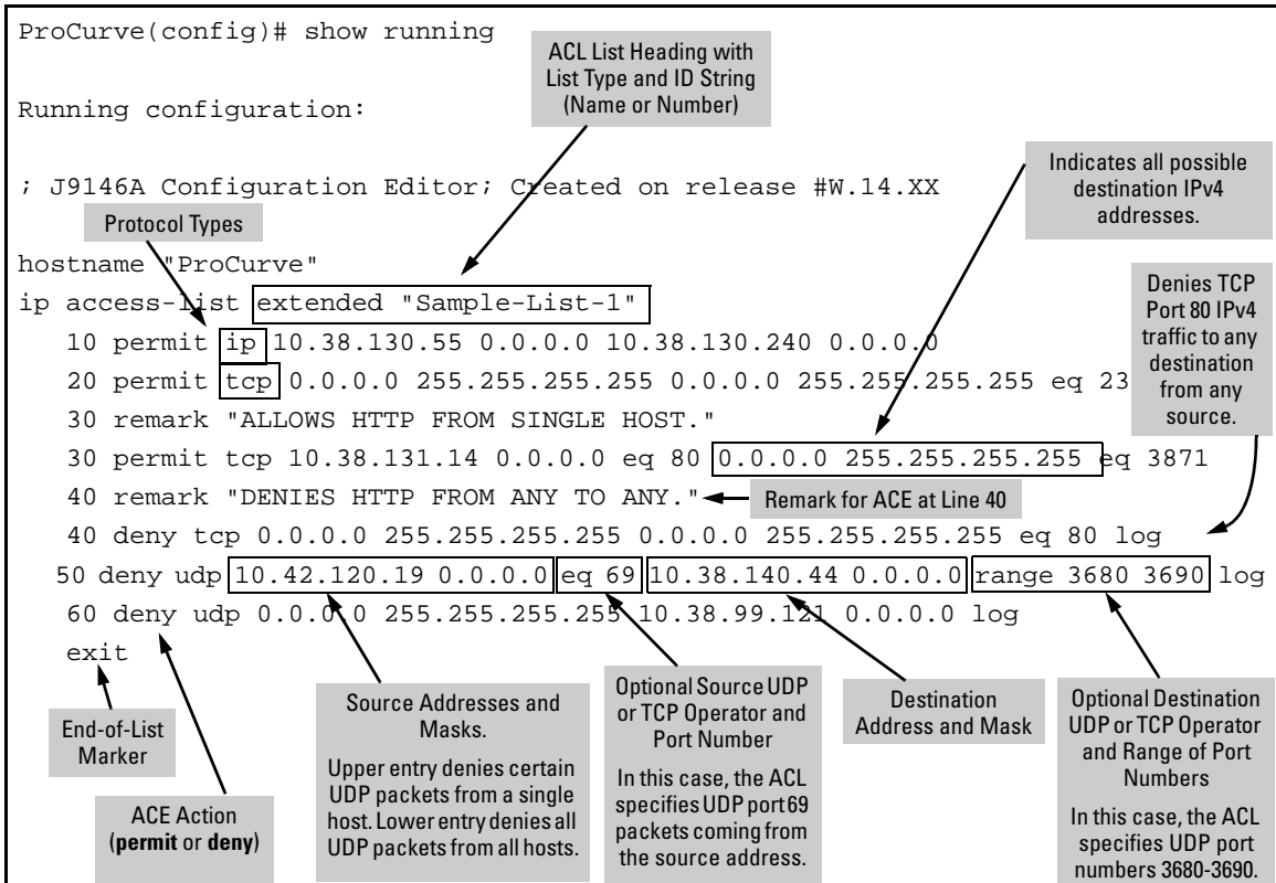
Figure 9-9. Example of a Displayed Extended ACL Configuration
